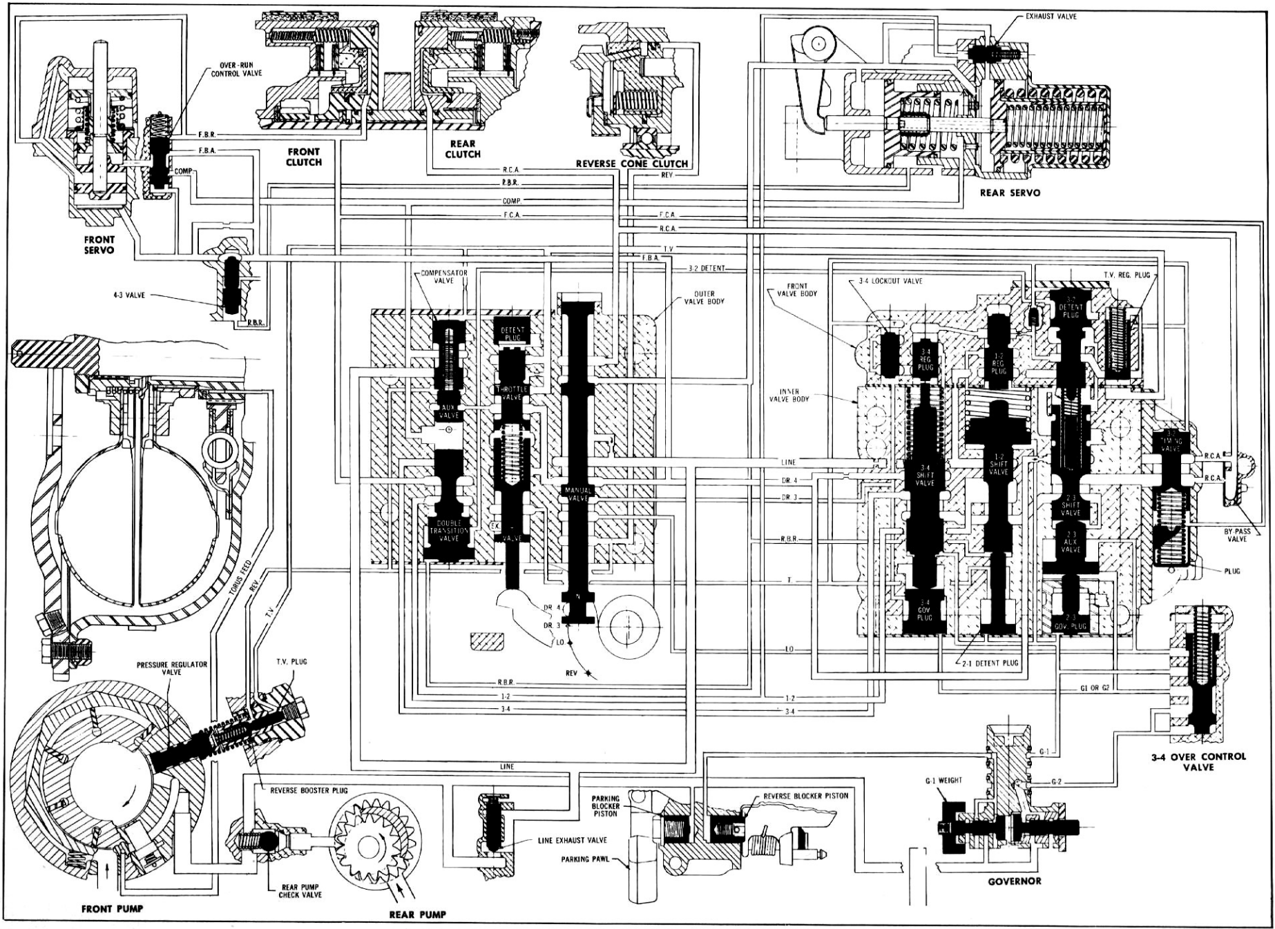
Fig. 14-3 Hydra-Matic Transmission Oil Circuit
