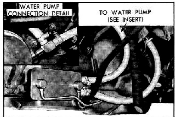
Fig. 14-6 Oil Cooler Hose and Pipe Connections
